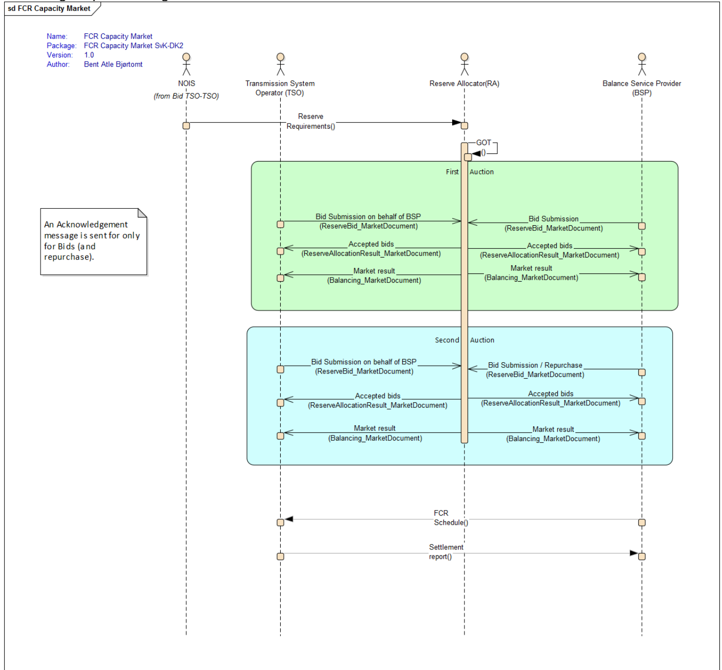
Figure 2 Sequence diagram for the FCR capacity market, SE and DK2
