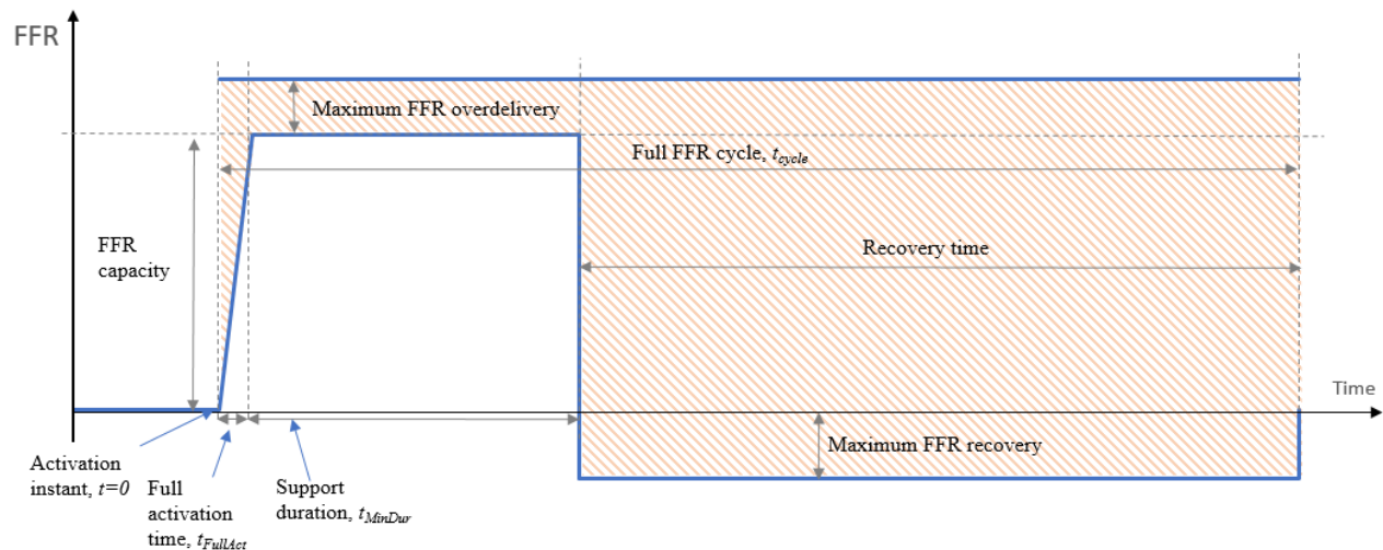
Figure 2: FFR recovery requirement for long duration FFR.
