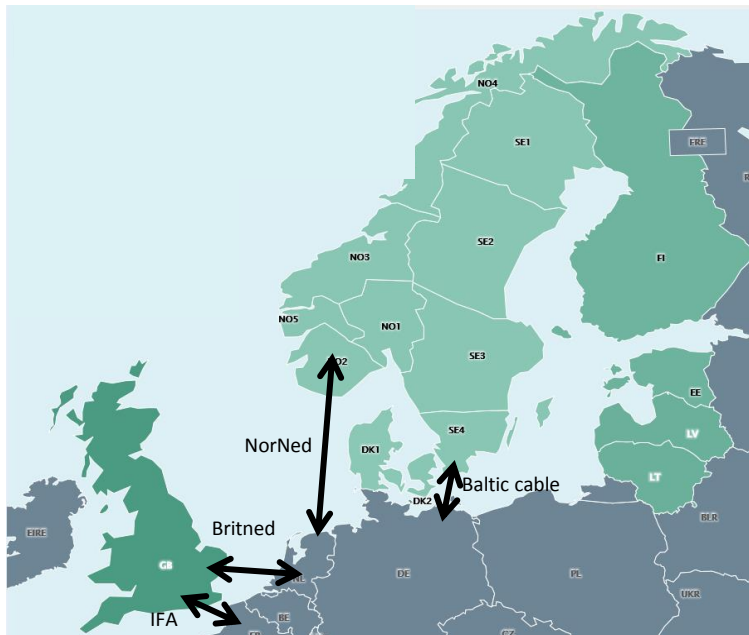
Figure 1. Interconnectors where implicit grid losses are implemented today; IFA (GB-FR), Britned (GB-NL), NorNed (NO2-NL) and Baltic cable (SE4-DE).
